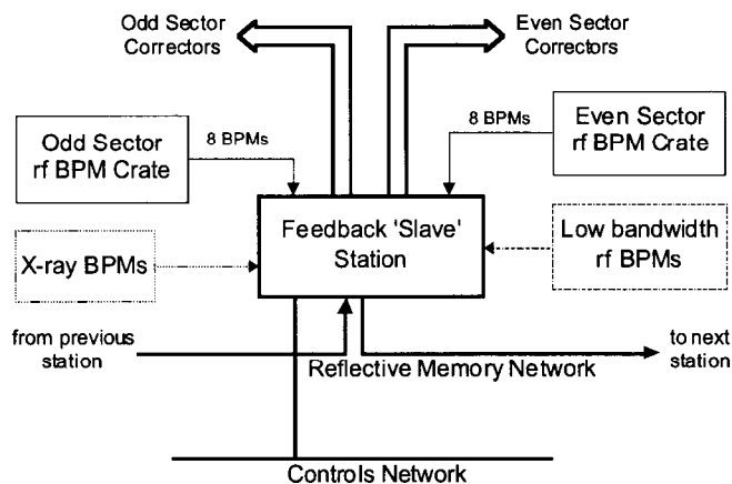
FIGURE 2. Real-time orbit feedback system layout.
