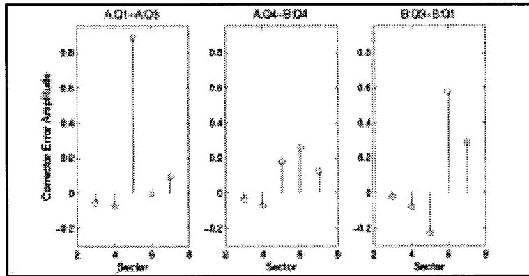
FIGURE 10. Horizontal corrector 'error' patterns for excitation of the ten different quadrupoles located in Sector 6.
