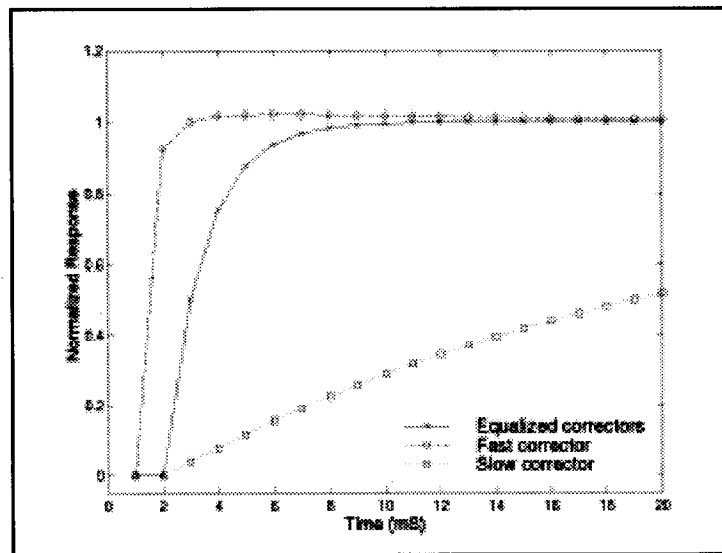
FIGURE 8. Equalized horizontal step response.
