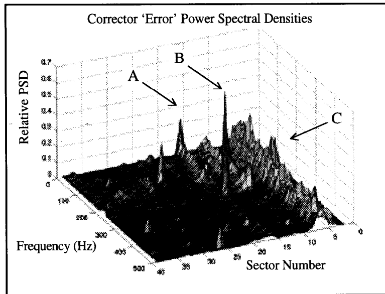
FIGURE 9. Example 'roadmap' of sources of horizontal orbit motion (see text for explanation of labeled features).
