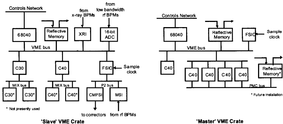
FIGURE 3. 'Master' and 'slave' crate components.
